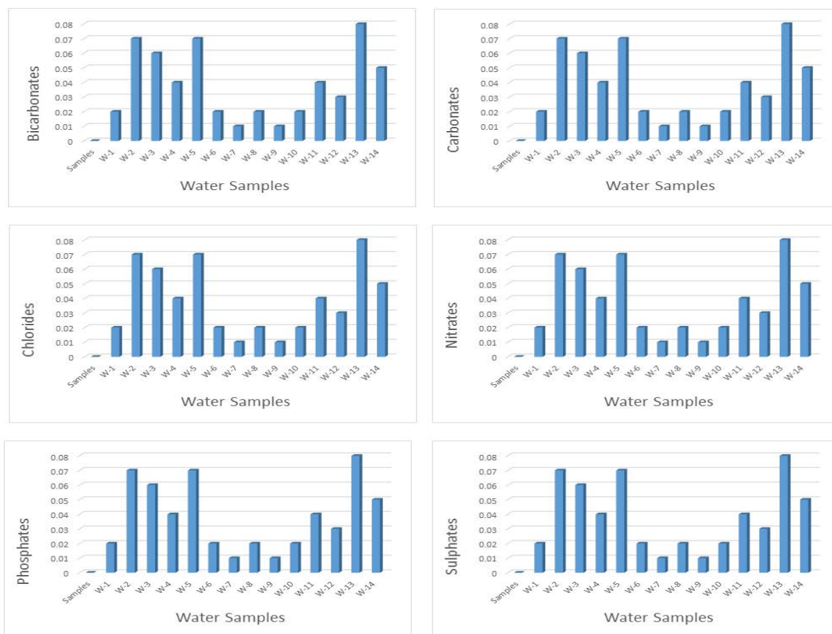
Fig. 2. Graphical representation of \text{HCO}_3^- , \text{CO}_3^{2-} , \text{Cl}^- , \text{NO}_3^- , \text{PO}_4^{3-} and \text{SO}_4^{2-} ions in tested water samples
