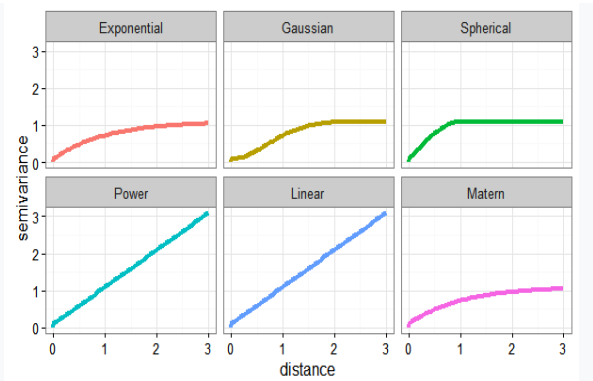
Fig. 2 Variogram models.
