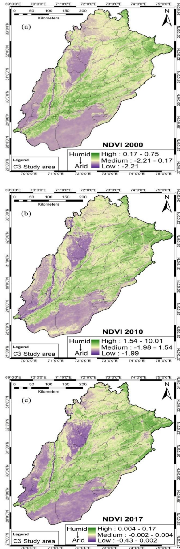
Fig. 2 Map showing classification of NDVI index over Punjab based on pixel data (a) Year 2000 (b) Year 2010 and (c) Year 2017 (Data Source: USGS Earth Explorer).
