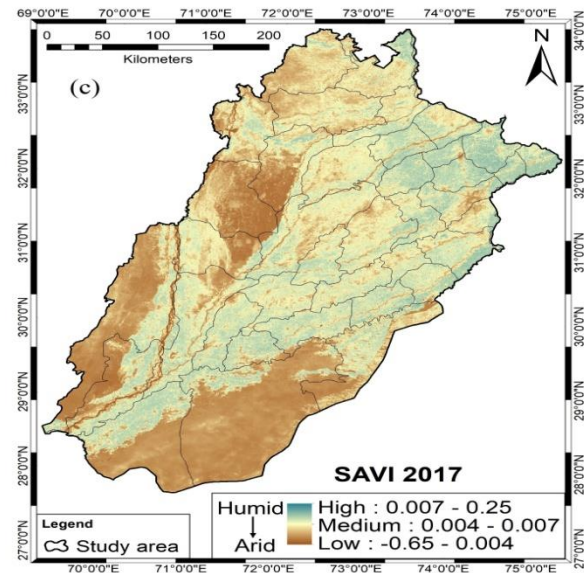
Fig. 3 Map showing classification of SAVI index over Punjab based on pixel data (a) Year 2000 (b) Year 2010 and (c) Year 2017 (Data Source: USGS Earth Explorer).
