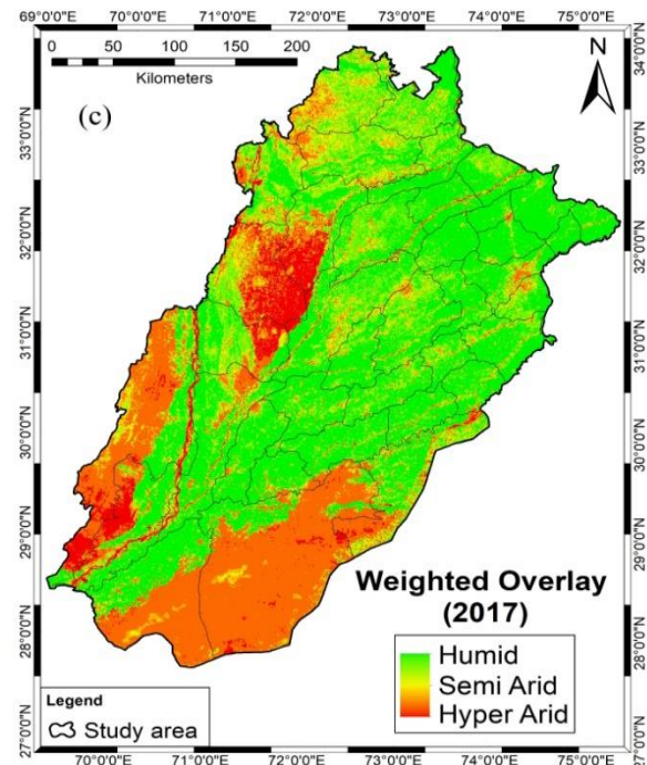
Fig. 6 Map showing classification of aridity over Punjab based on weighted overlay of NDVI, SAVI and TNDVI index by using pixel data (a) Year 2000 (b) Year 2010 and (c) Year 2017 (Data Source: USGS Earth Explorer).
