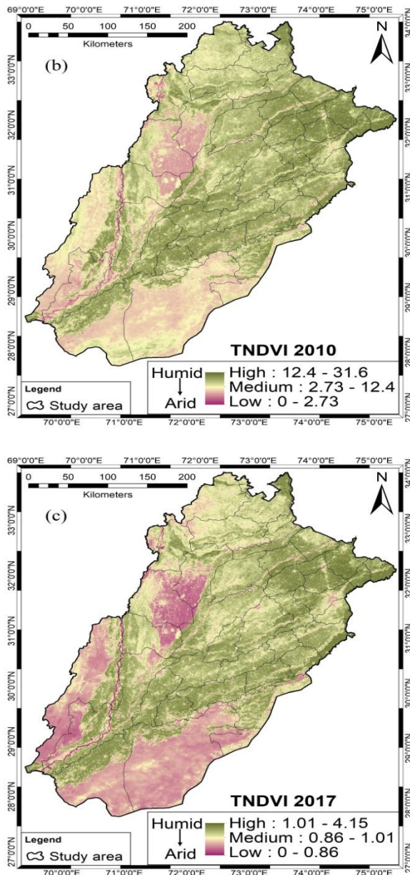
Fig. 4 Map showing classification of TNDVI index over Punjab based on pixel data (a) Year 2000 (b) Year 2010 and (c) Year 2017 (Data Source: USGS Earth Explorer).
