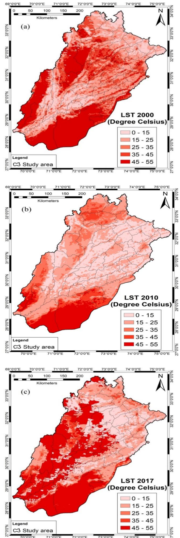
Fig. 5 Map showing classification of LST over Punjab based on pixel data (a) Year 2000 (b) Year 2010 and (c) Year 2017 (Data Source: USGS Earth Explorer).
