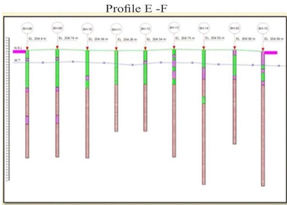
Fig. 6 Borehole soil profile E to F.
