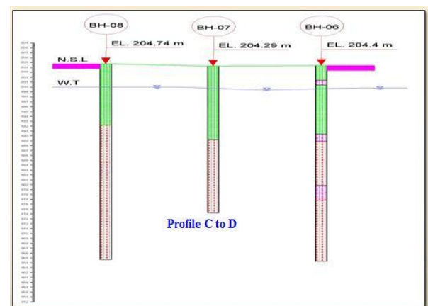
Fig. 5 Borehole soil profile C to D.
