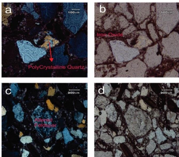
Fig. 5 (Mag: 100X): Polycrystalline quartz in the centre of photomicrograph. Microcrystalline calcite is developed along the grain contacts of quartz (A, B); angular, quartz poor, calcite rich, have floating texture. In the centre a grain of alkali feldspar is partially altered to clays probably into kaolinite, illite/smectite. The bioclasts in the form of lithics are scattered throughout of the slides (C, D).
