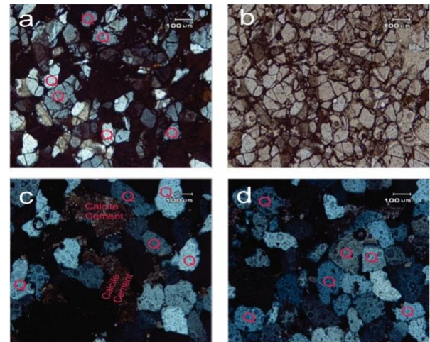
Fig. 3 (Mag: 100X for A, B, and 40X for C, D): (A, B) Intensive fracturing within the quartz grains; (C) Microcrystalline cement replacing quartz margins; (D) suture grain contacts showing compaction and dissolution.
