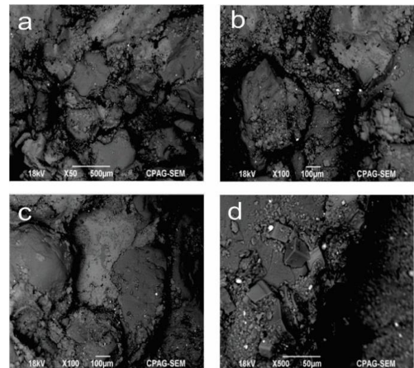
Fig. 13 SEM images of sample B-8. Two types of calcite along with quartz are present, which are mostly fractured and generated various kinds of channels ranging from 5-10 \mu\text{m} and generated secondary porosity and permeability.
