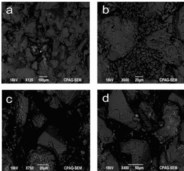
Fig. 8 Sample # A-4. Scanning Electron Microscope (SEM) images where the main constituent is quartz and its fracturing is very high as is evident in B, where the grain size is less than 10 \mu\text{m} . Secondary porosity and permeability is also visible along with the overgrowth of quartz itself (C, D).
