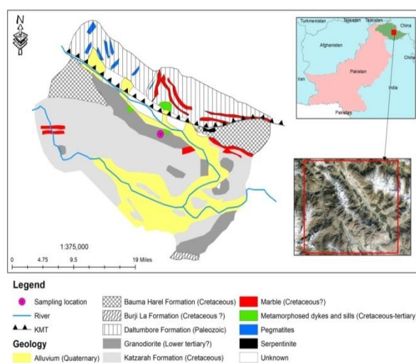
Fig. 1 Geological map of Shigar valley, Baltistan, Pakistan (after Hanson, 1988, 1989).
