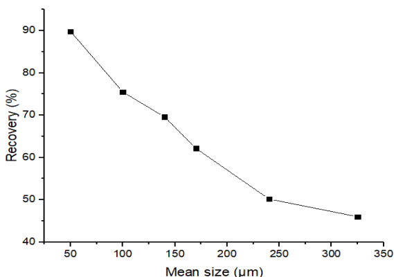
Fig. 5 Recovery of copper as a function of particle size.
