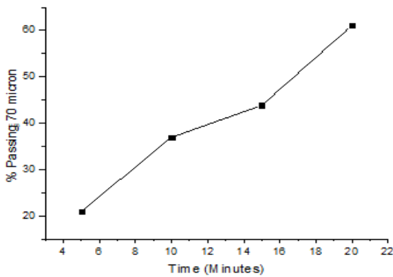
Fig. 4 Effect of grinding time on particle size.
