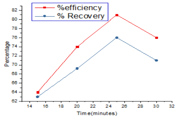
Fig. 7 Recovery of copper as a function of grinding time
