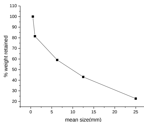
Fig. 2. Particle size curve for jaw crusher
