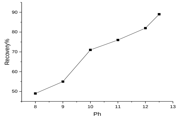
Fig. 6 Recovery of copper as a function pH.
