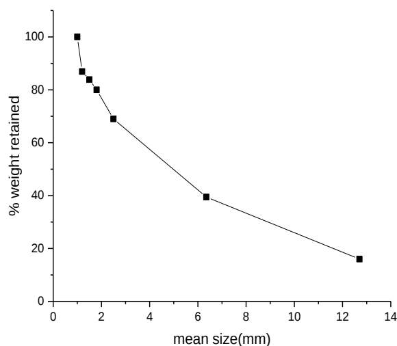
Fig. 3 Particle size curve for roll crusher.
