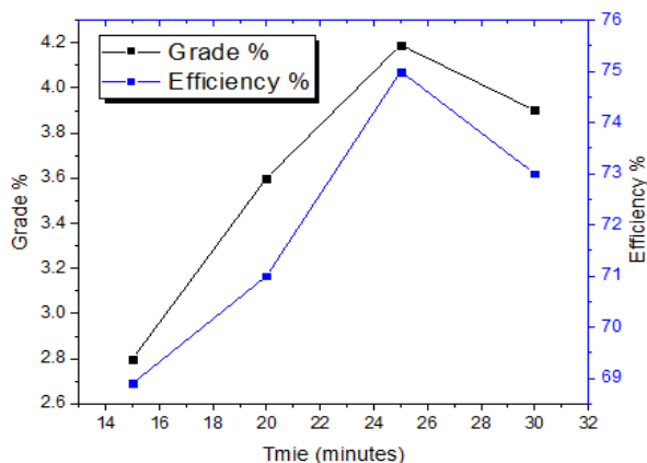
Fig. 8 Effect of grinding time on grade.
