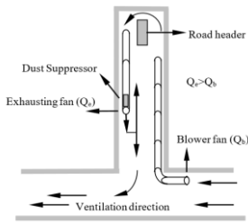
Fig. 1a. Recirculating ventilation system in the heading of main and tailgates
