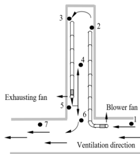
Figure 2. Measuring points
