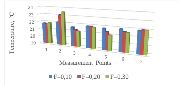
Fig. 3c. Temperature change according to different "F" values
