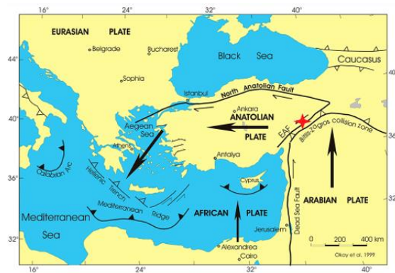
Fig. 2 Tectonic plates around Türkiye .
